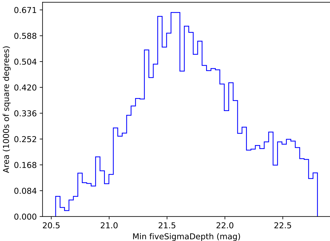
too_elab_r8_d3_gz_v3.4_10yrs WFD i band: Min fiveSigmaDepth
