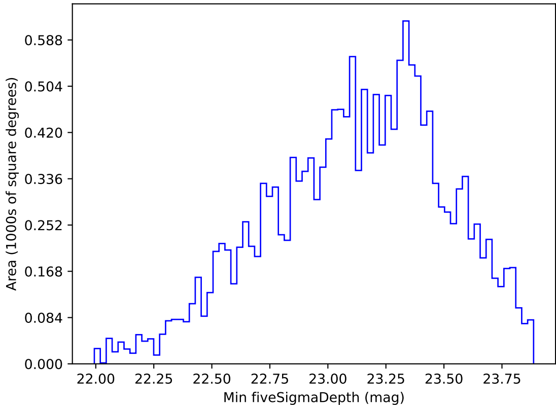
too_elab_r8_d3_gz_v3.4_10yrs WFD g band: Min fiveSigmaDepth
