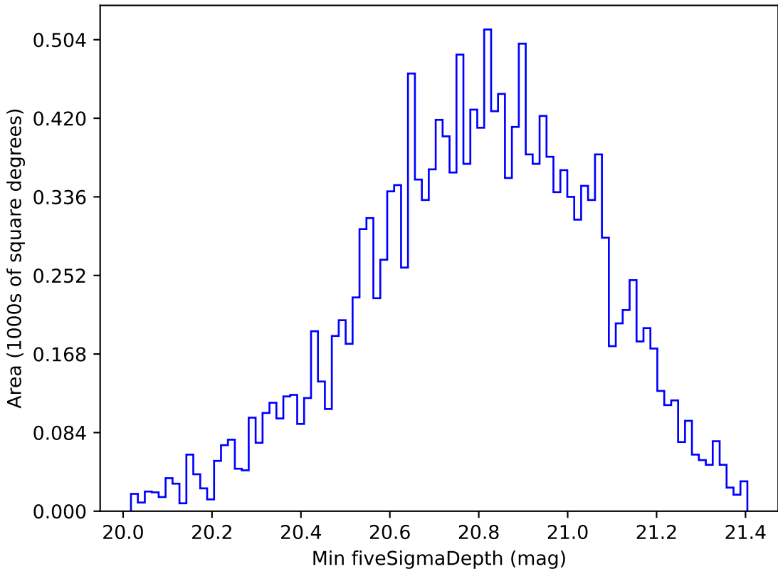
too_elab_r8_d3_gz_v3.4_10yrs WFD all bands: Min fiveSigmaDepth
