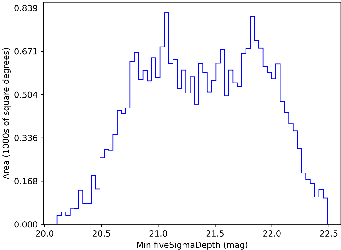
too_elab_r8_d3_gz_v3.4_10yrs All sky z band: Min fiveSigmaDepth
