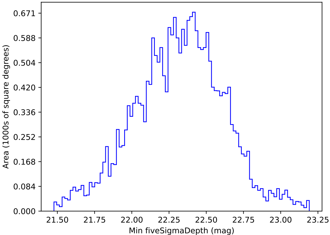
too_elab_r8_d3_gz_v3.4_10yrs All sky u band: Min fiveSigmaDepth
