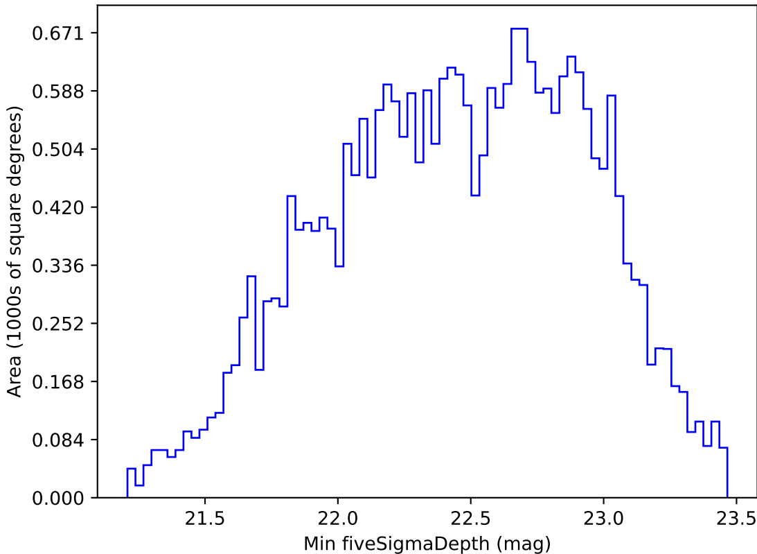
too_elab_r8_d3_gz_v3.4_10yrs All sky r band: Min fiveSigmaDepth
