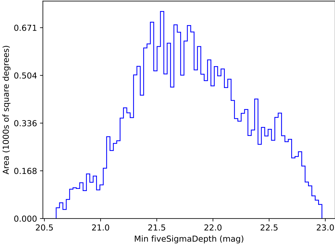
too_elab_r8_d3_gz_v3.4_10yrs All sky i band: Min fiveSigmaDepth
