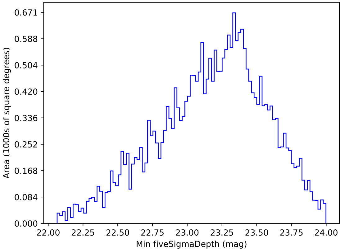
too_elab_r8_d3_gz_v3.4_10yrs All sky g band: Min fiveSigmaDepth
