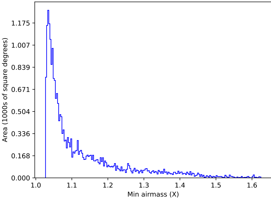
too_elab_r8_d3_gz_v3.4_10yrs Yr 1 y band: Min airmass
