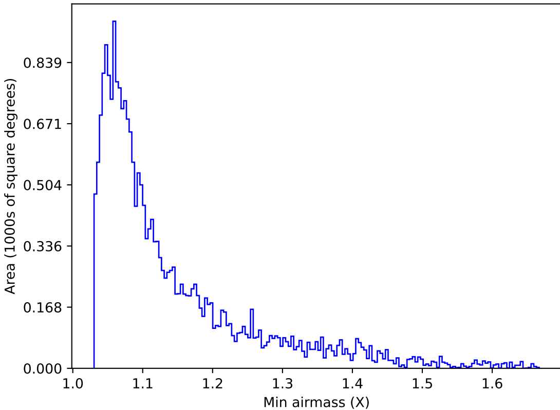
too_elab_r8_d3_gz_v3.4_10yrs Yr 1 u band: Min airmass
