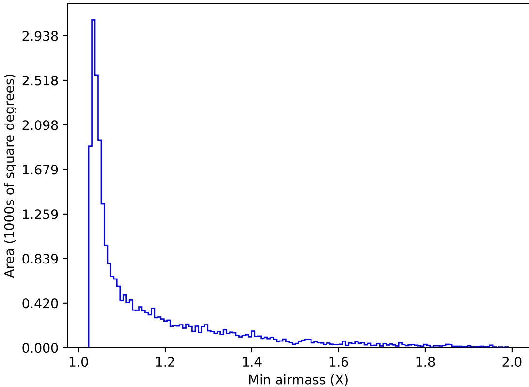
too_elab_r8_d3_gz_v3.4_10yrs Yr 1 r band: Min airmass
