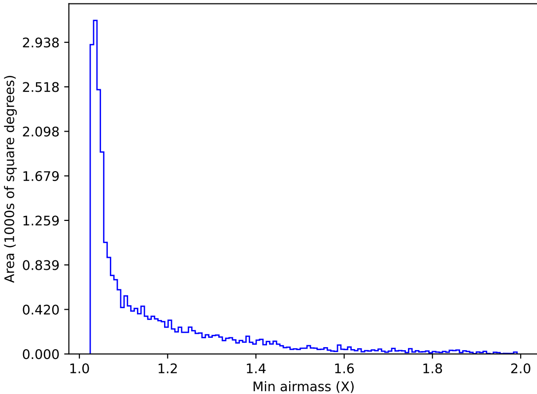
too_elab_r8_d3_gz_v3.4_10yrs Yr 1 i band: Min airmass
