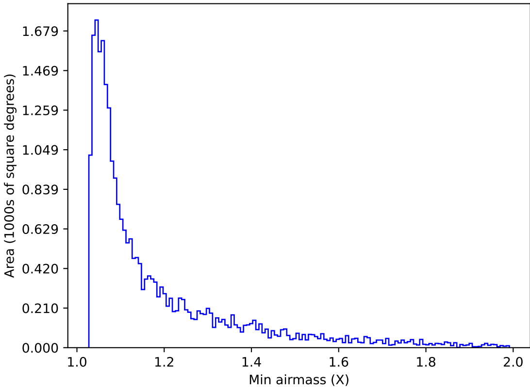
too_elab_r8_d3_gz_v3.4_10yrs Yr 1 g band: Min airmass
