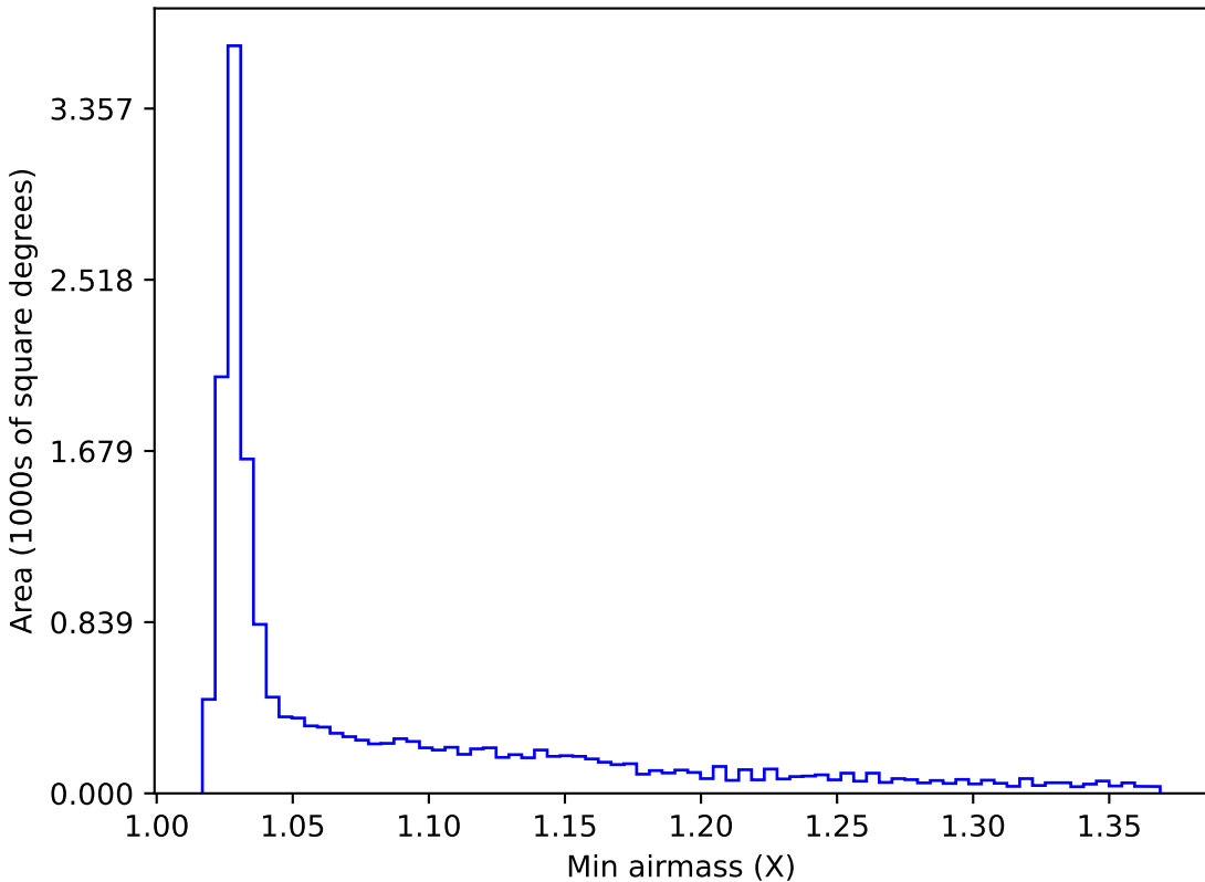
too_elab_r8_d3_gz_v3.4_10yrs WFD z band: Min airmass
