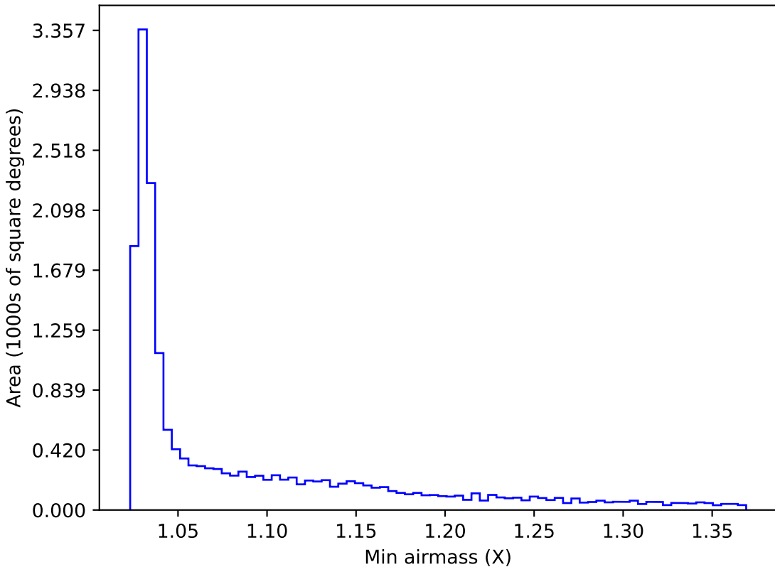
too_elab_r8_d3_gz_v3.4_10yrs WFD y band: Min airmass
