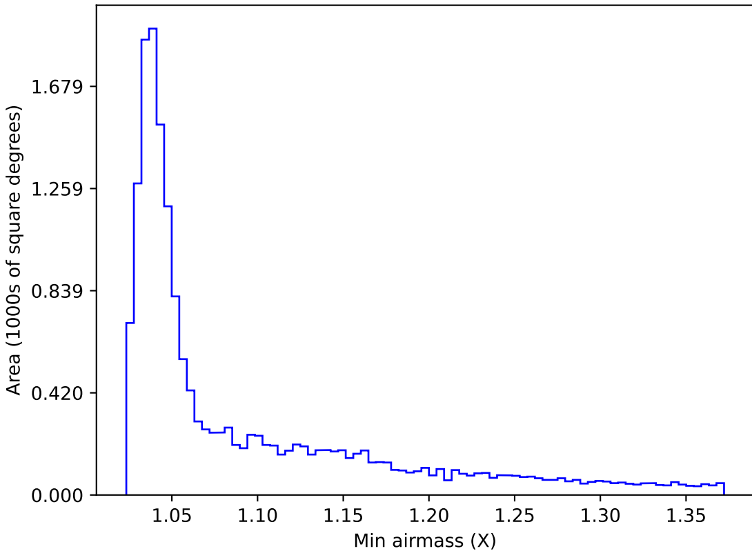
too_elab_r8_d3_gz_v3.4_10yrs WFD u band: Min airmass
