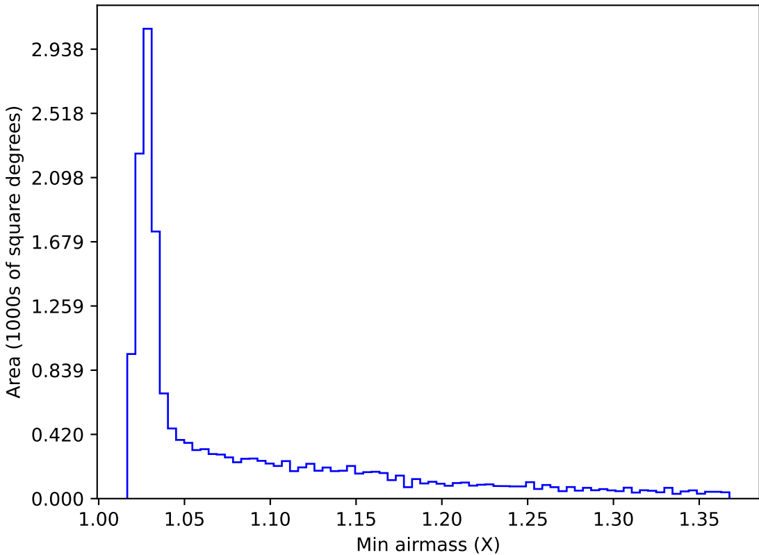
too_elab_r8_d3_gz_v3.4_10yrs WFD r band: Min airmass
