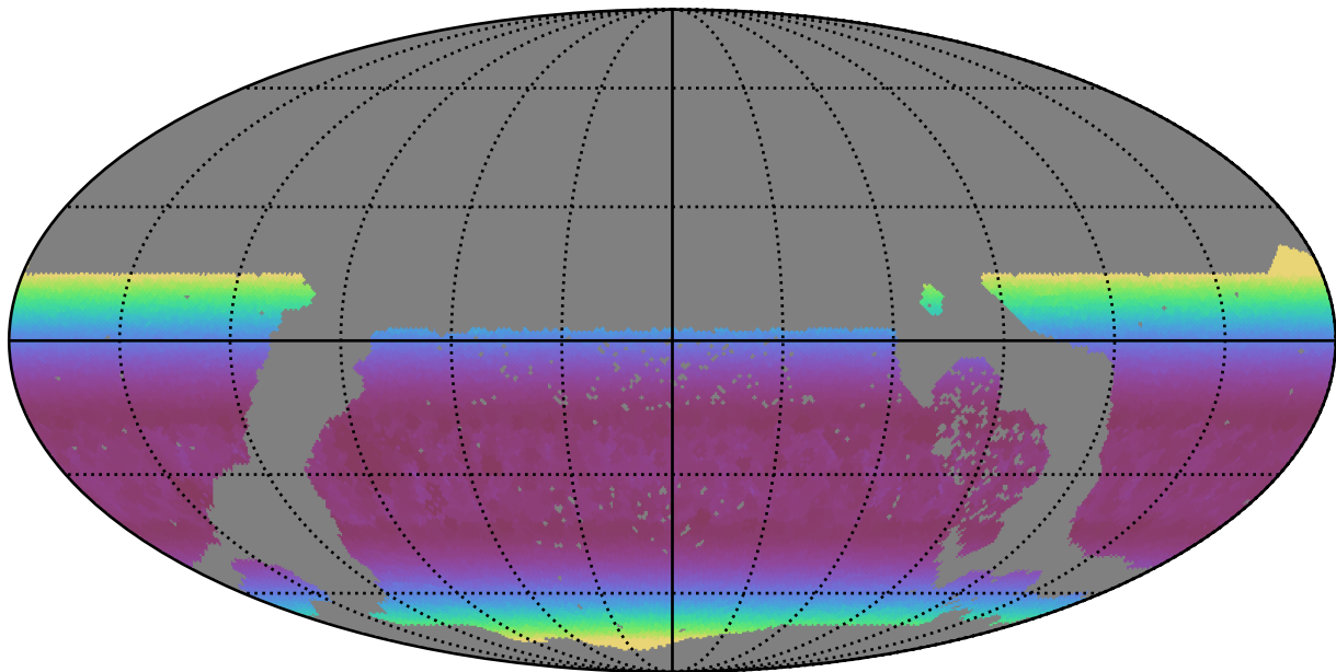
too_elab_r8_d3_gz_v3.4_10yrs WFD g band: Min airmass
