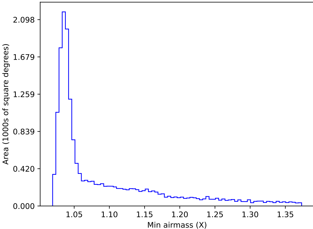
too_elab_r8_d3_gz_v3.4_10yrs WFD g band: Min airmass
