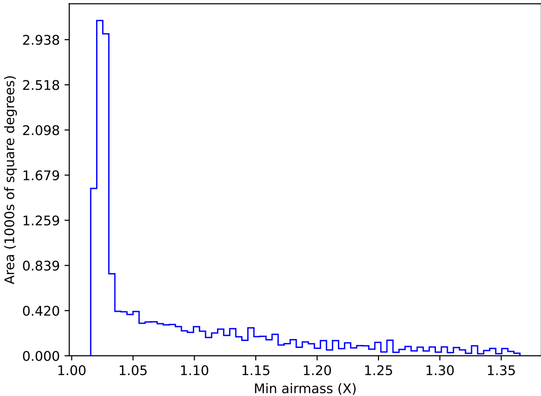
too_elab_r8_d3_gz_v3.4_10yrs WFD all bands: Min airmass
