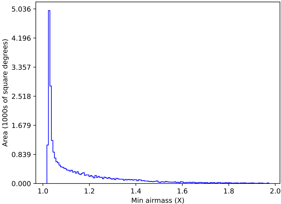
too_elab_r8_d3_gz_v3.4_10yrs All sky z band: Min airmass
