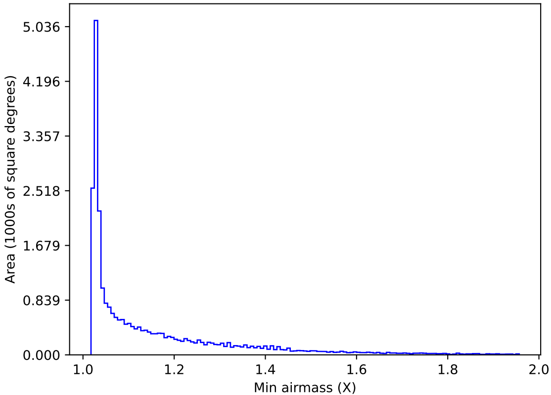
too_elab_r8_d3_gz_v3.4_10yrs All sky r band: Min airmass
