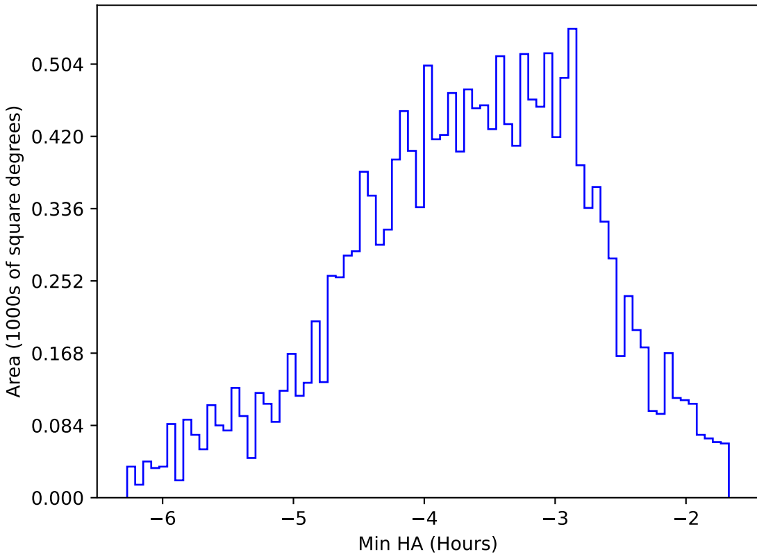
too_elab_r8_d3_gz_v3.4_10yrs WFD y band: Min HA
