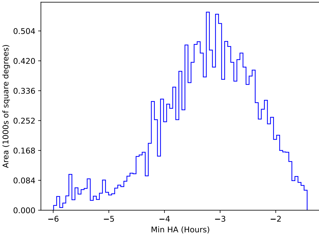
too_elab_r8_d3_gz_v3.4_10yrs WFD u band: Min HA
