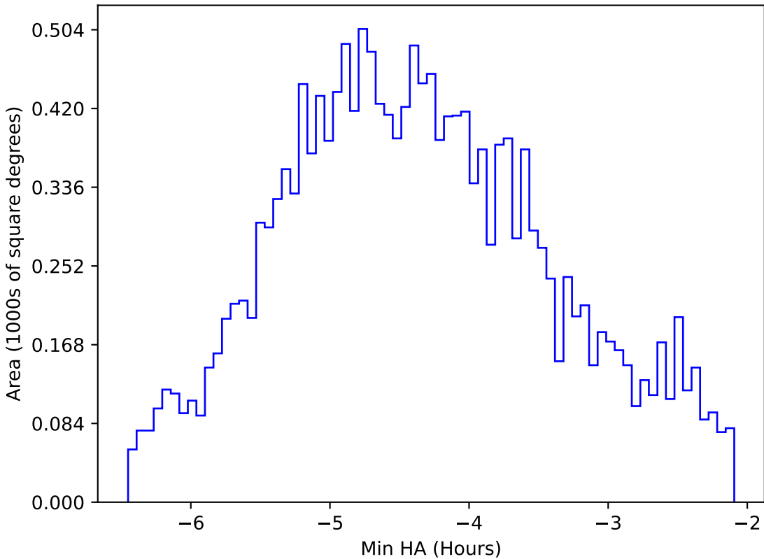
too_elab_r8_d3_gz_v3.4_10yrs WFD i band: Min HA
