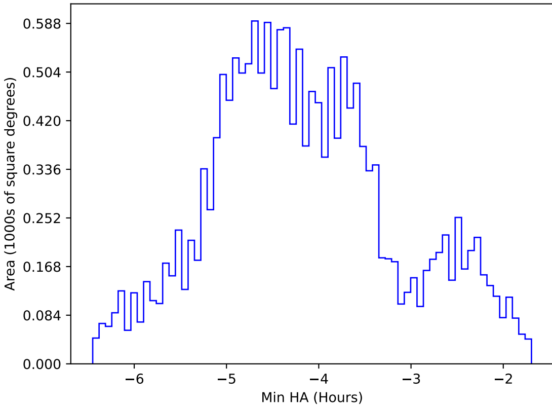
too_elab_r8_d3_gz_v3.4_10yrs WFD g band: Min HA
