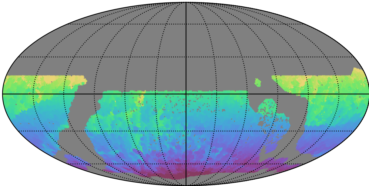
too_elab_r8_d3_gz_v3.4_10yrs WFD all bands: Min HA
