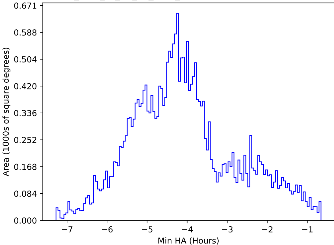
too_elab_r8_d3_gz_v3.4_10yrs All sky z band: Min HA
