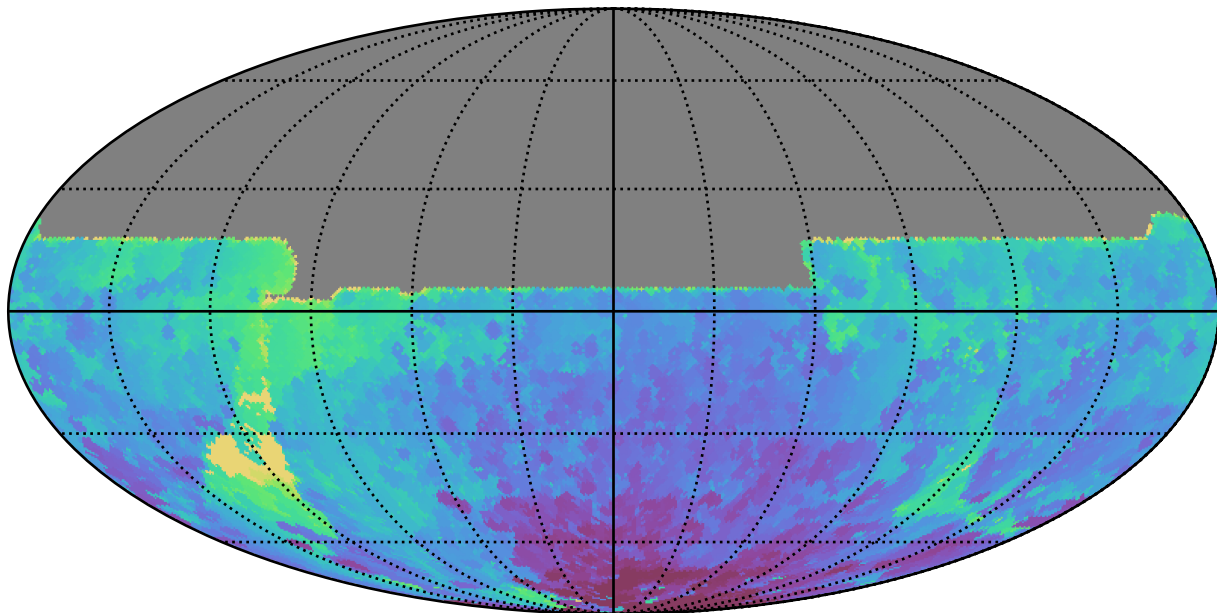
too_elab_r8_d3_gz_v3.4_10yrs All sky y band: Min HA
