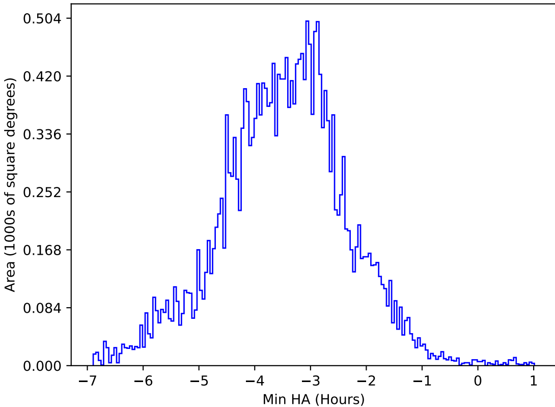
too_elab_r8_d3_gz_v3.4_10yrs All sky y band: Min HA
