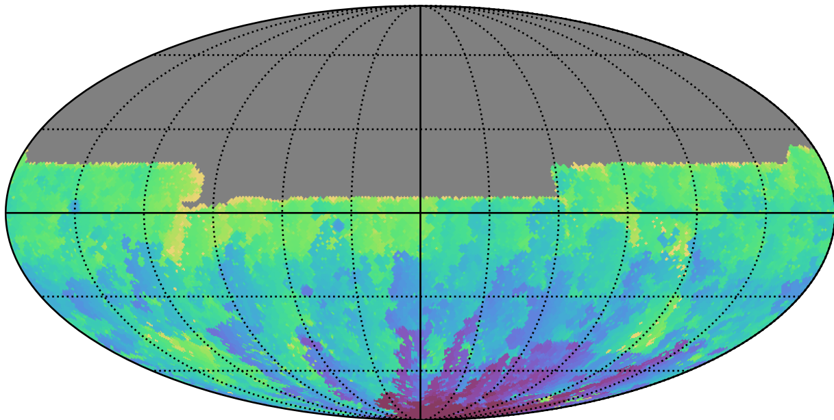
too_elab_r8_d3_gz_v3.4_10yrs All sky u band: Min HA
