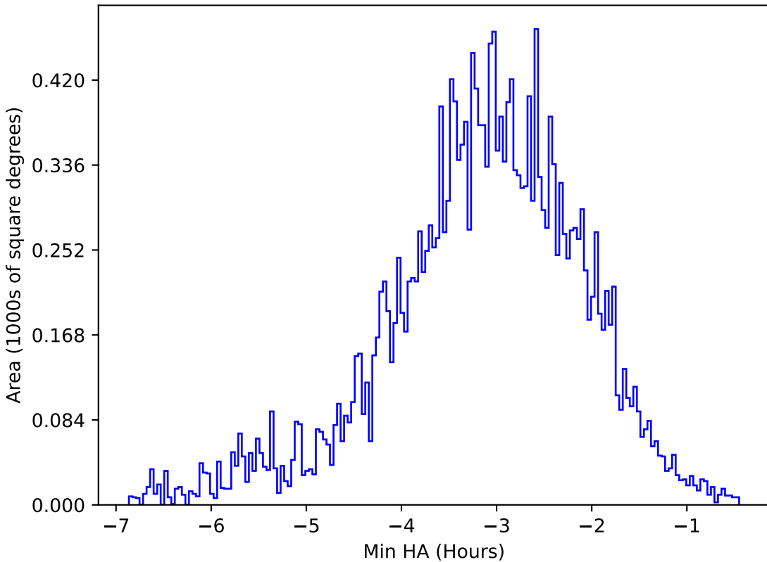
too_elab_r8_d3_gz_v3.4_10yrs All sky u band: Min HA
