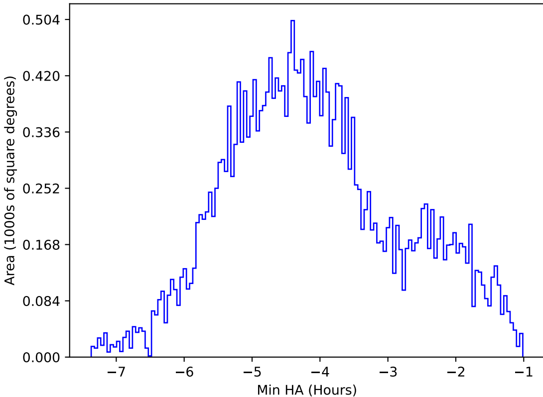
too_elab_r8_d3_gz_v3.4_10yrs All sky i band: Min HA
