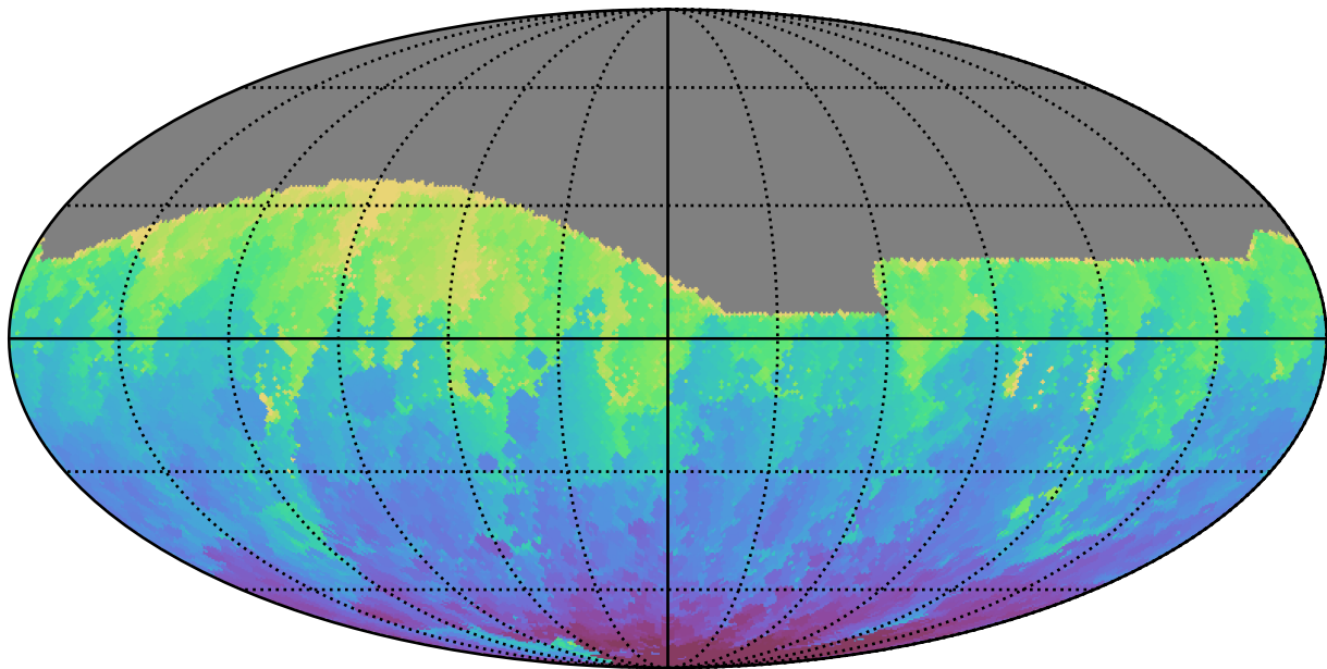
too_elab_r8_d3_gz_v3.4_10yrs All sky g band: Min HA
