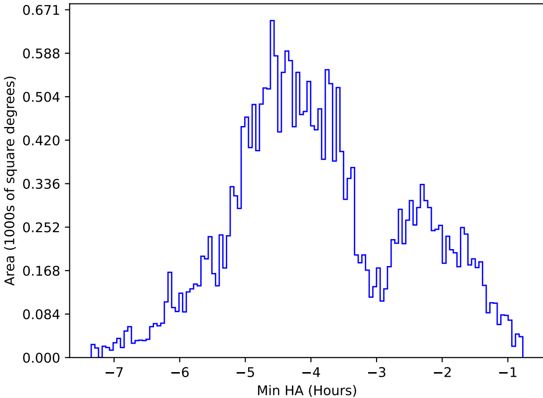
too_elab_r8_d3_gz_v3.4_10yrs All sky g band: Min HA
