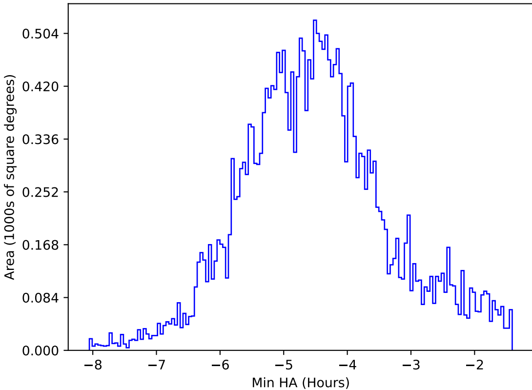
too_elab_r8_d3_gz_v3.4_10yrs All sky all bands: Min HA
