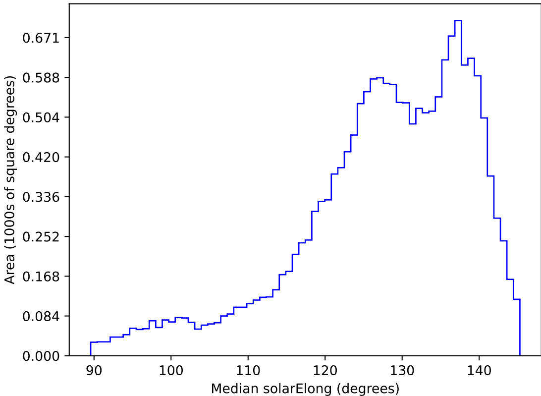
too_elab_r8_d3_gz_v3.4_10yrs WFD z band: Median solarElong
