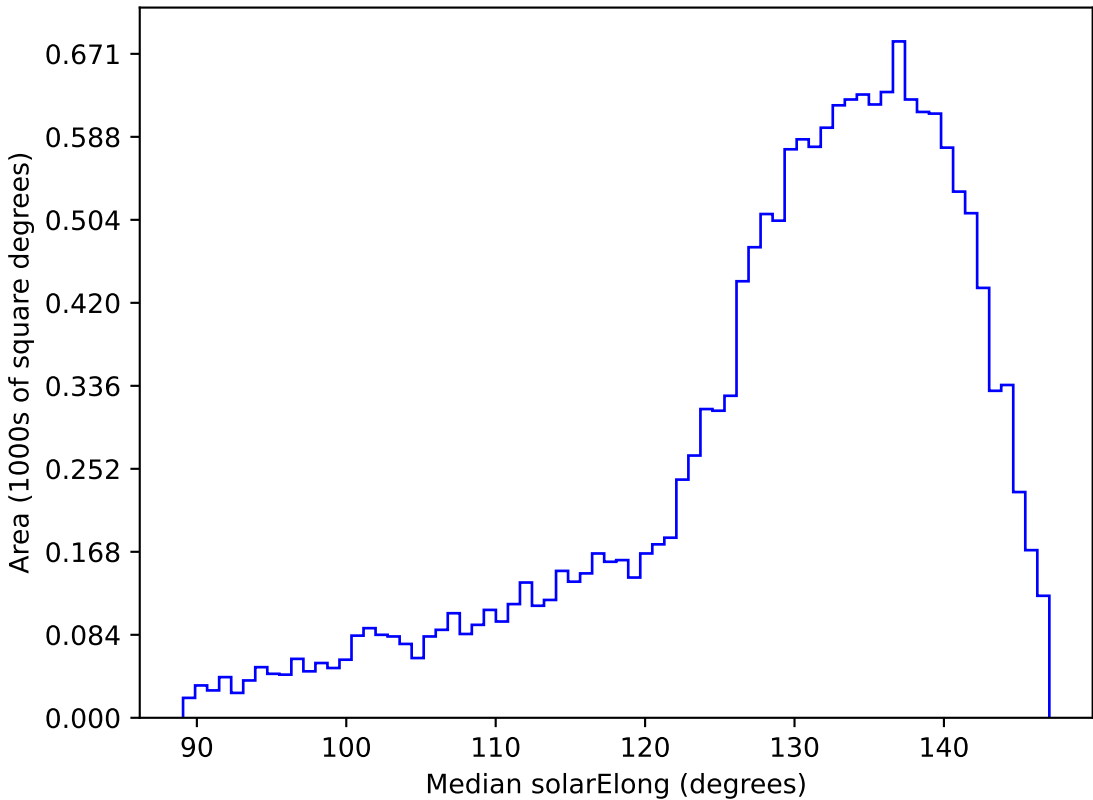
too_elab_r8_d3_gz_v3.4_10yrs WFD y band: Median solarElong
