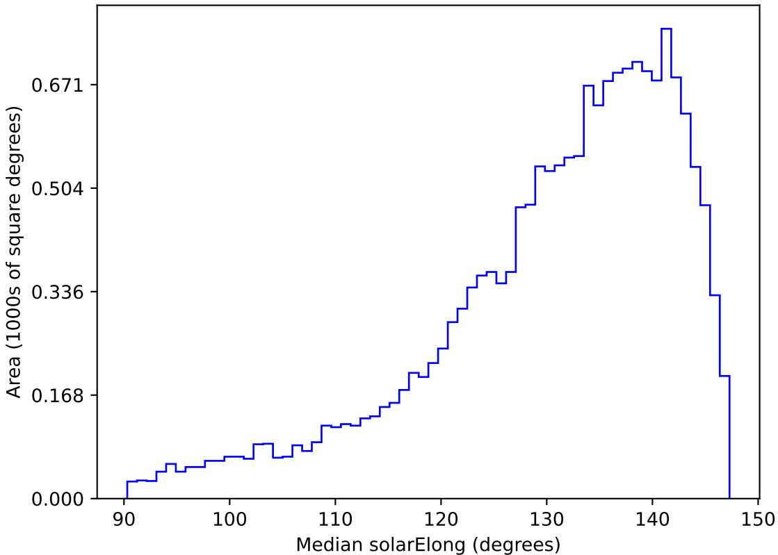
too_elab_r8_d3_gz_v3.4_10yrs WFD r band: Median solarElong
