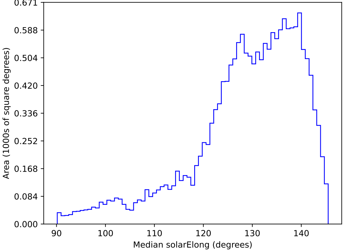
too_elab_r8_d3_gz_v3.4_10yrs WFD i band: Median solarElong
