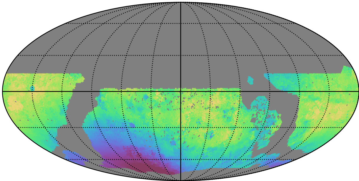
too_elab_r8_d3_gz_v3.4_10yrs WFD g band: Median solarElong
