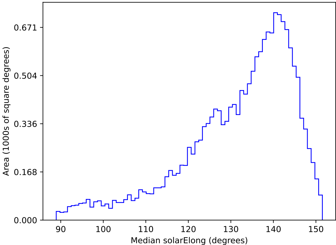
too_elab_r8_d3_gz_v3.4_10yrs WFD g band: Median solarElong
