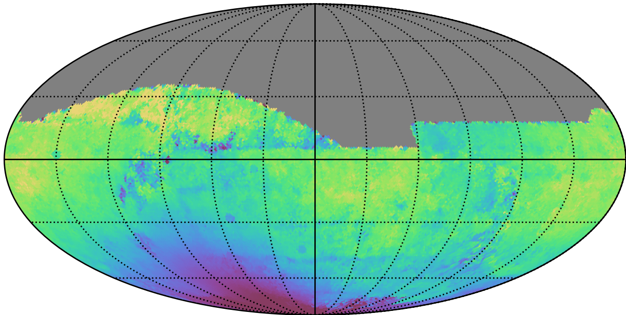
too_elab_r8_d3_gz_v3.4_10yrs All sky z band: Median solarElong
