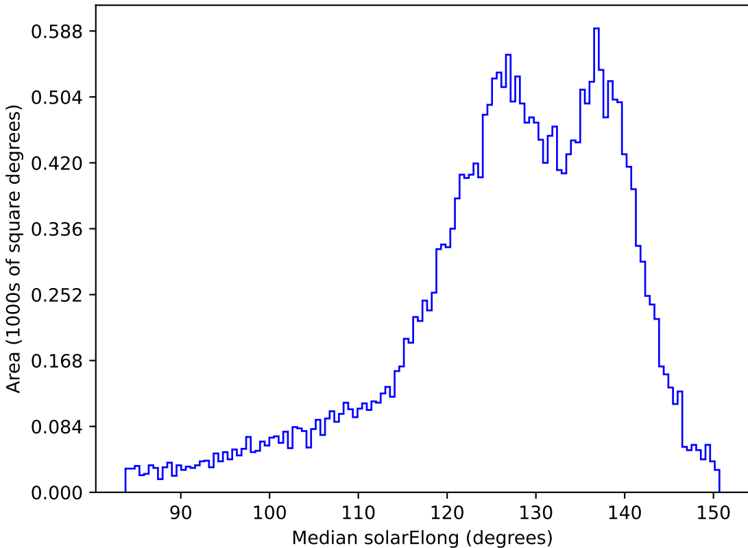
too_elab_r8_d3_gz_v3.4_10yrs All sky z band: Median solarElong
