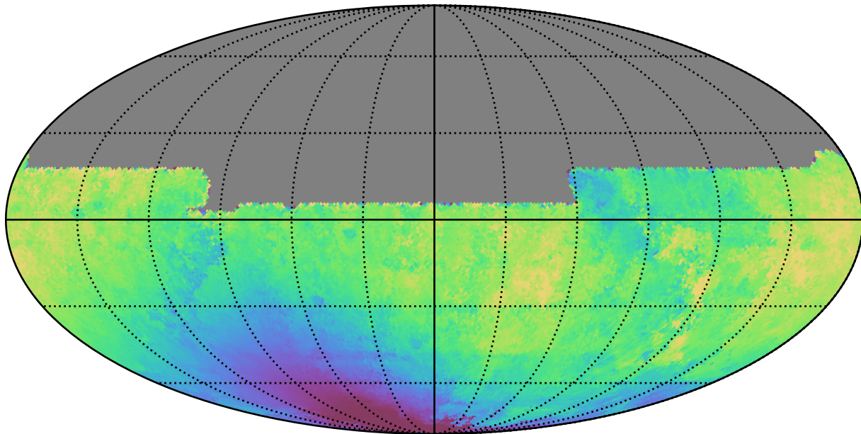
too_elab_r8_d3_gz_v3.4_10yrs All sky y band: Median solarElong
