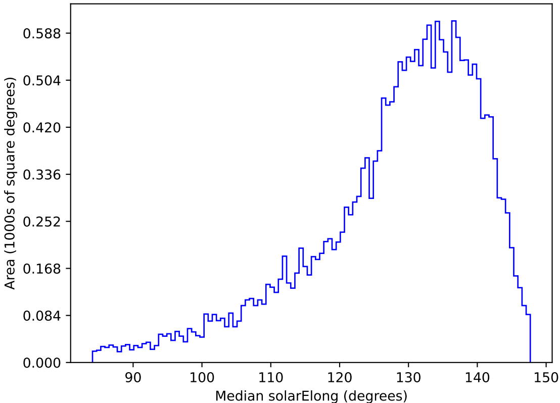
too_elab_r8_d3_gz_v3.4_10yrs All sky y band: Median solarElong
