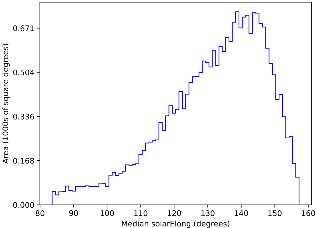
too_elab_r8_d3_gz_v3.4_10yrs All sky u band: Median solarElong
