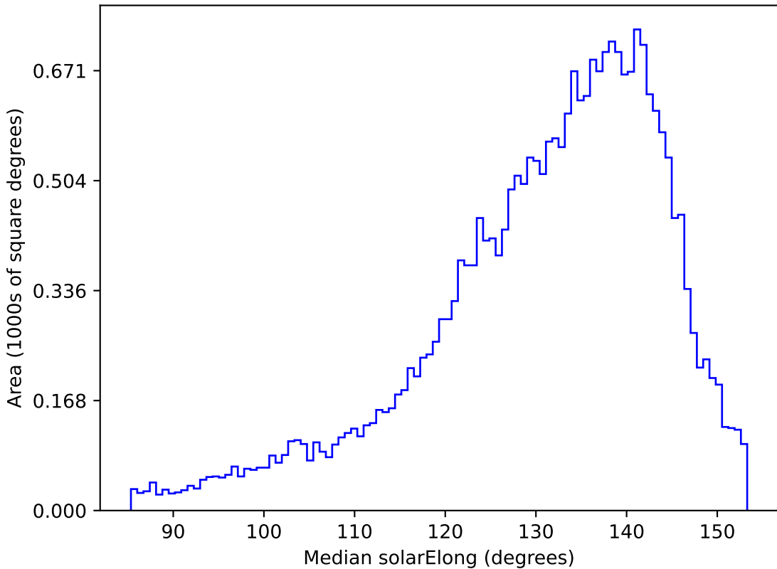
too_elab_r8_d3_gz_v3.4_10yrs All sky r band: Median solarElong
