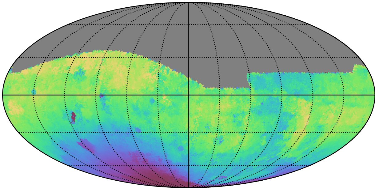
too_elab_r8_d3_gz_v3.4_10yrs All sky g band: Median solarElong
