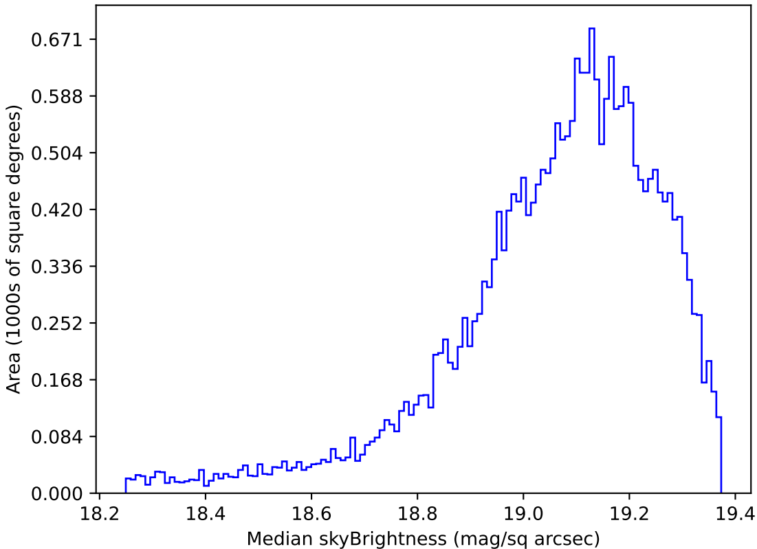
too_elab_r8_d3_gz_v3.4_10yrs Yr 1 z band: Median skyBrightness
